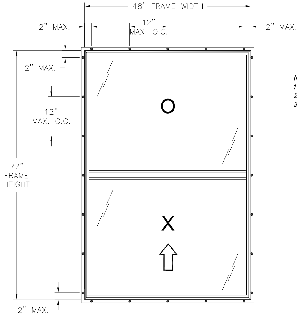
400/475 VINYL SINGLE HUNG TILT WINDOW EXTERIOR VIEW
