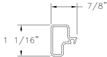
MEETING RAIL REINFORCEMENT (203-A) ALUMINUM 6063-T5
