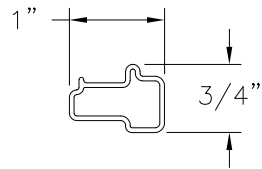
LOCK RAIL REINFORCEMENT (204-B) ALUMINUM 6063-T5
